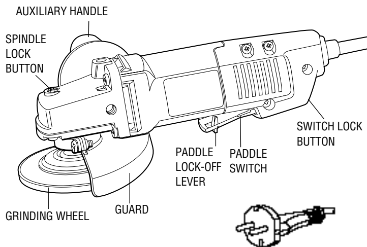
2750-220 4-1/2" Angle Grinder with 220 volt plug
