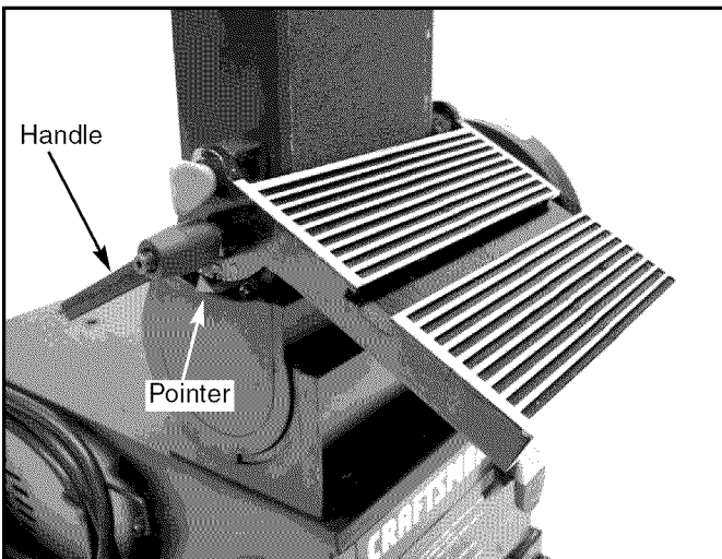
Figure 12 - Table Tilts Down 45°
