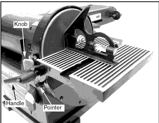
Figure 5 – Using Table with Disc
