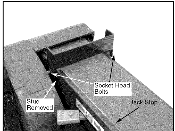
Figure 13 - Attaching the Back Stop
