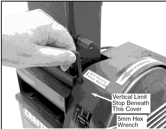
Figure 11 - Loosen Bolt to Tilt Belt Assembly
