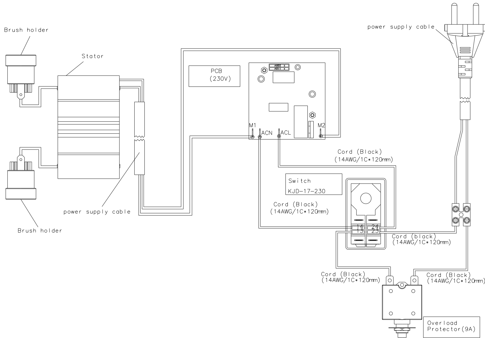
CONNECTION DIAGRAM 5140034-89 BLACK & DECKER (U.S.) INC. PRODUCT SERVICE DIVISION TOWSON, MARYLAND (Jun06-TS)
